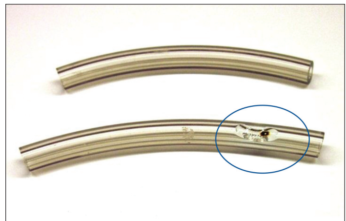
Close-up photo of a part damaged by the heat generated during curing. The photo compares parts exposed to conventional (bottom) and LED (top) light-curing energy sources.
