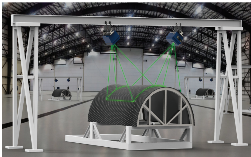
Two Tracer M projectors projecting onto an engine nacelle for ply layup in a composites clean room.
