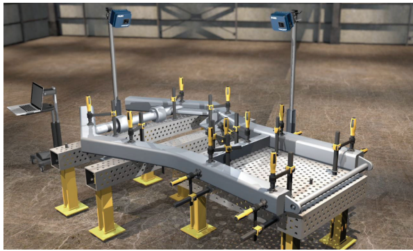
Two Tracer M projectors at work in an assembly operation.
